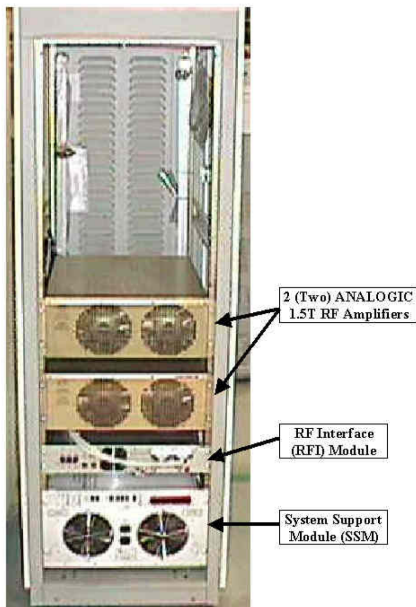
1.5T SRF CABINET ILLUSTRATION 1-1
